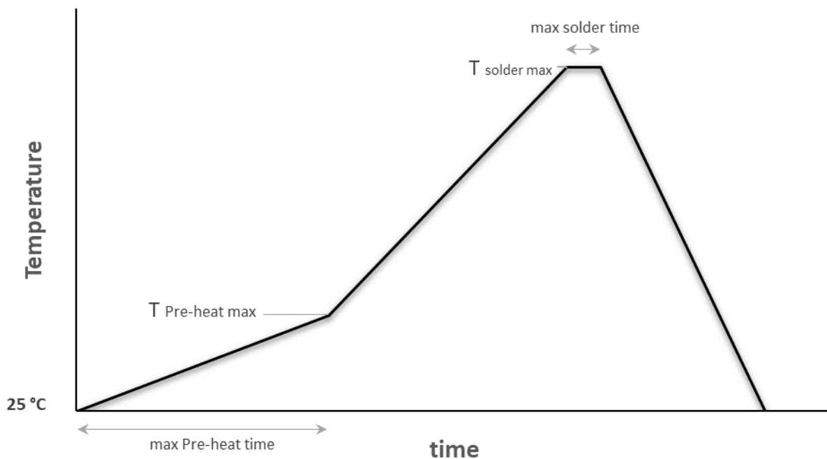
Soldering Temperature Profile
