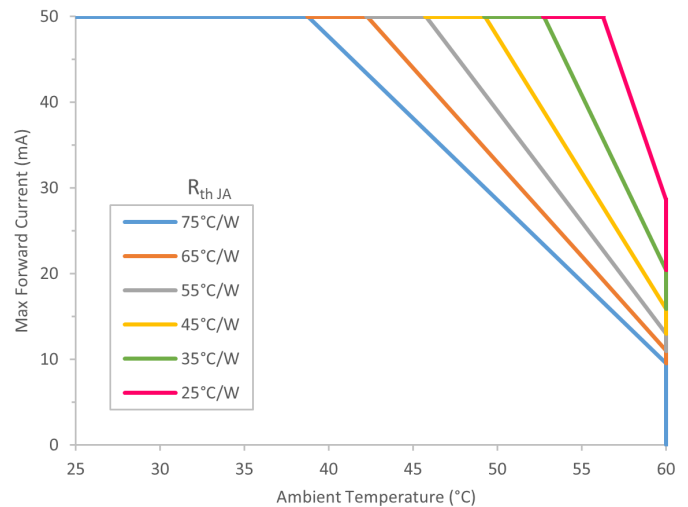
Figure 9. Max Forward current de-rating
